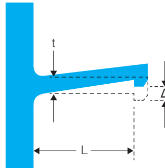
Figure 32: Snap fit design parameters
