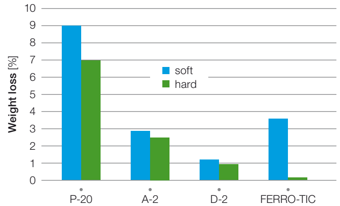
Figure 13: Wear resistance of surface treatments
