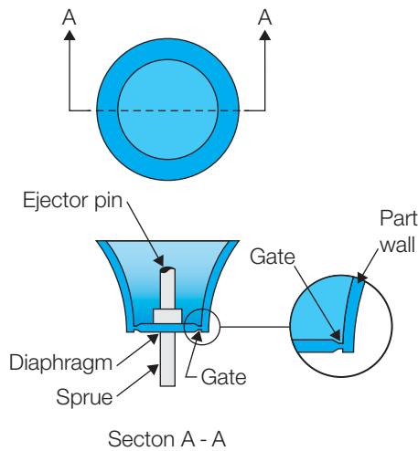
Figure 23: Diaphragm gate
